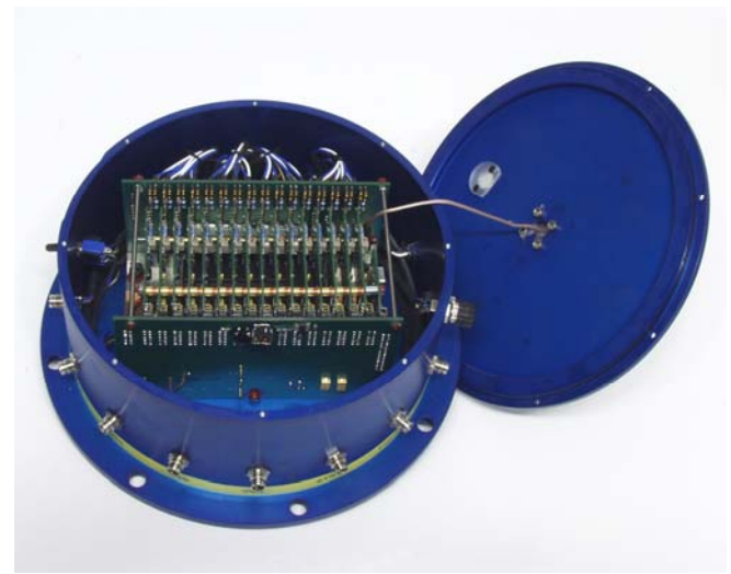
Encoder inside
